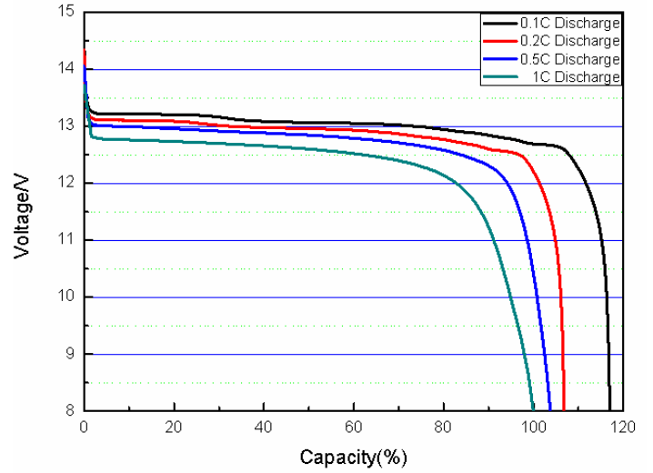
Discharge performance
